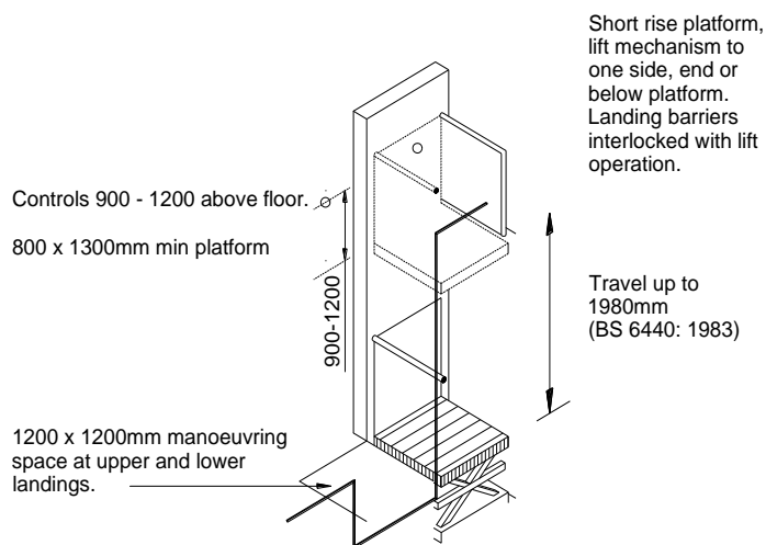
Vertical Platform Lift to BS 6440:1983
