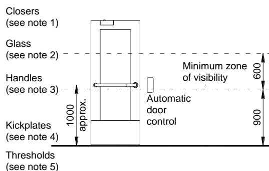
Typical Door Elevation
