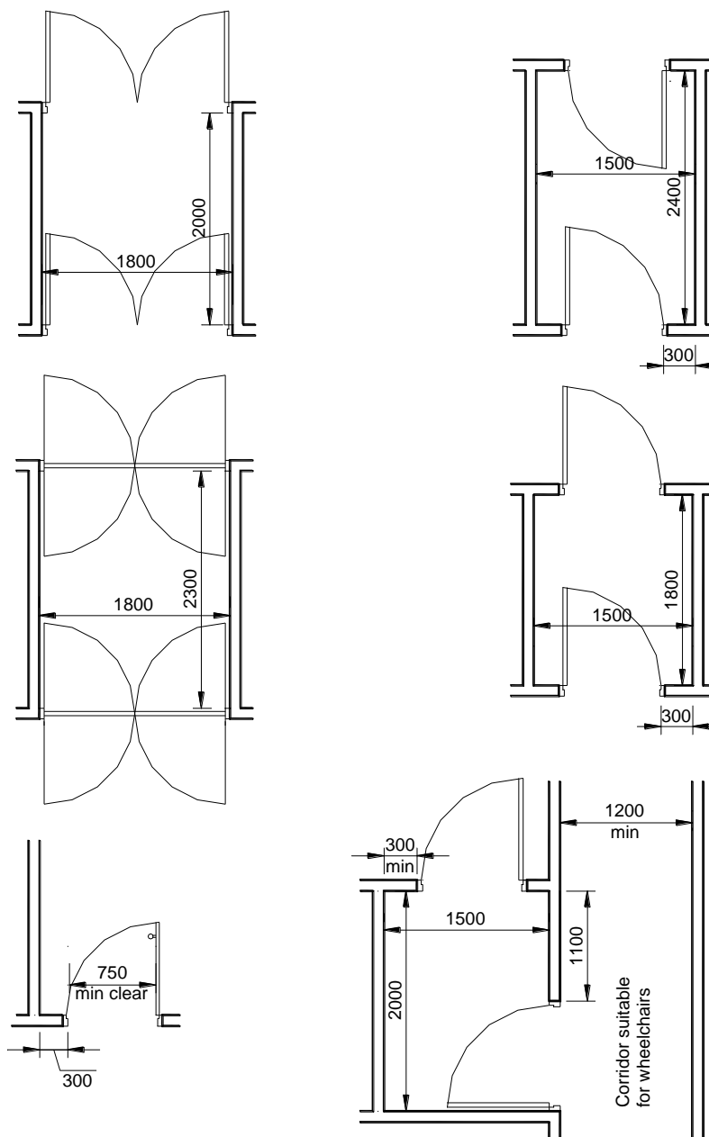
Plans of Typical Internal Lobby Arrangements
