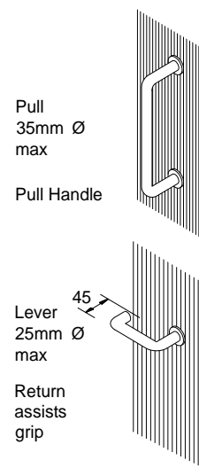
Typical Handle Details
