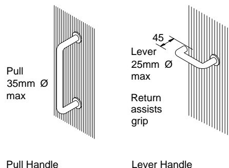
Typical Handle Details
