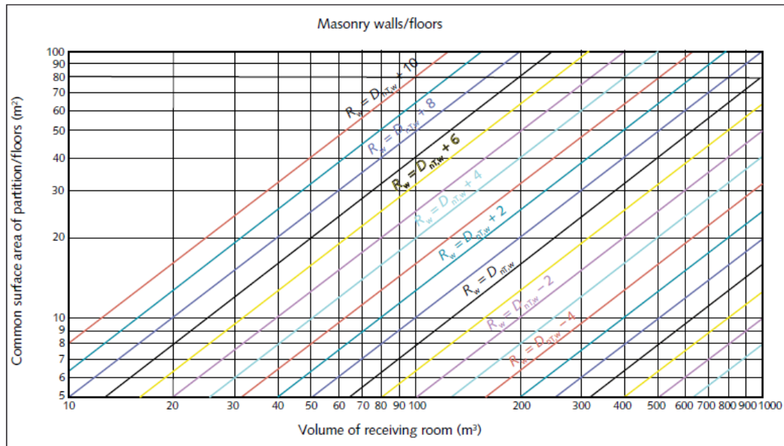
Figure A2: Calculation of R_w from D_{nT,w} for lightweight constructions
