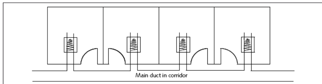
Figure 7: Typical room layout with main duct in corridor
