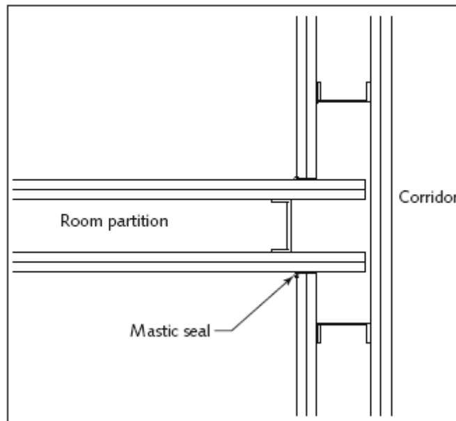
Figure 3: Typical schematic detail at junction of acoustic partitions with corridor walls (preferred)
