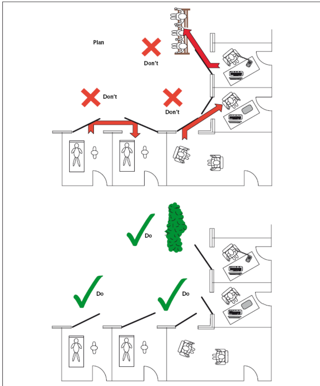
Figure 1: Reflected sound from openable windows
