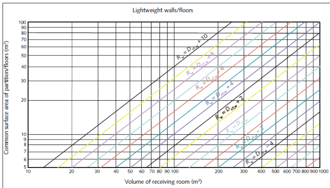
Figure A1: Calculation of R_w from D_{nT,w} for lightweight constructions
