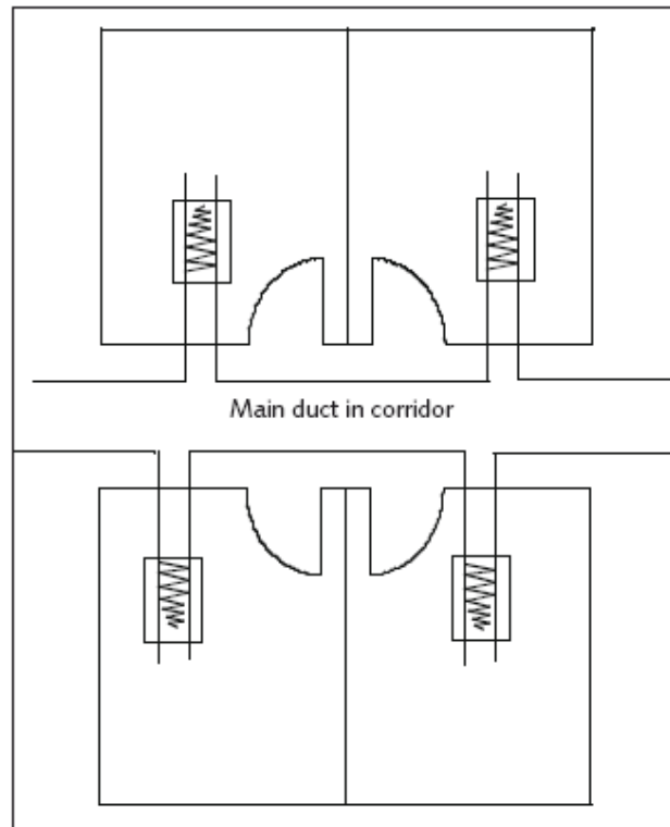
Figure 8: Typical room layout with rooms both sides of corridor duct
