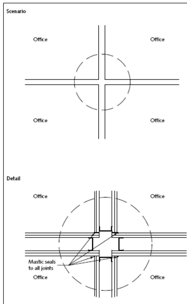
Figure 5: Typical schematic detail at junction of four acoustic partitions
