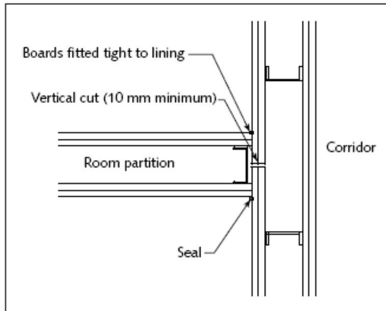
Figure 4: Typical schematic detail at junction of acoustic partitions with corridor walls
