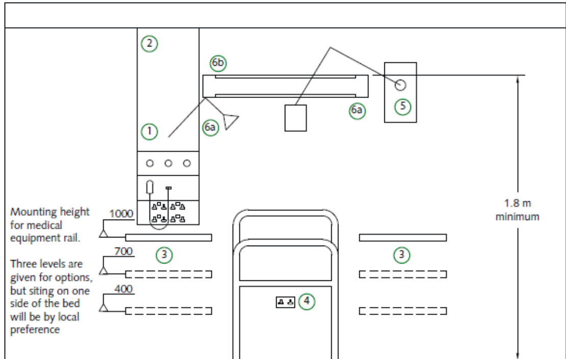
Figure B2: Vertical trunking.
