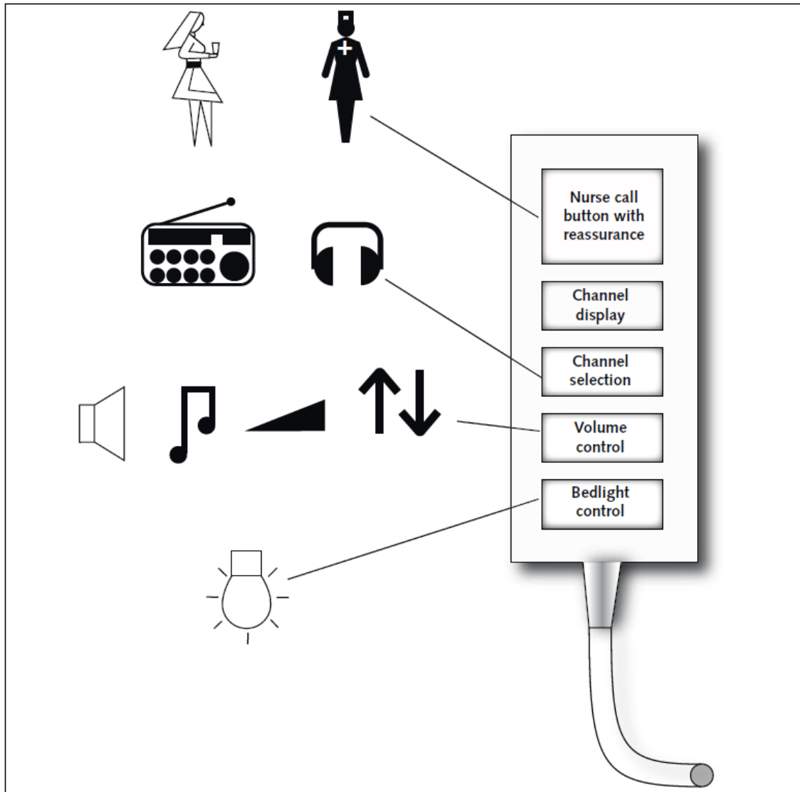
Figure 1: Typical layout of patient handset with example of symbols.
