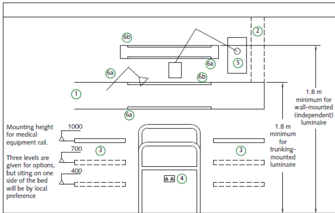
Figure B1: Horizontal trunking.
