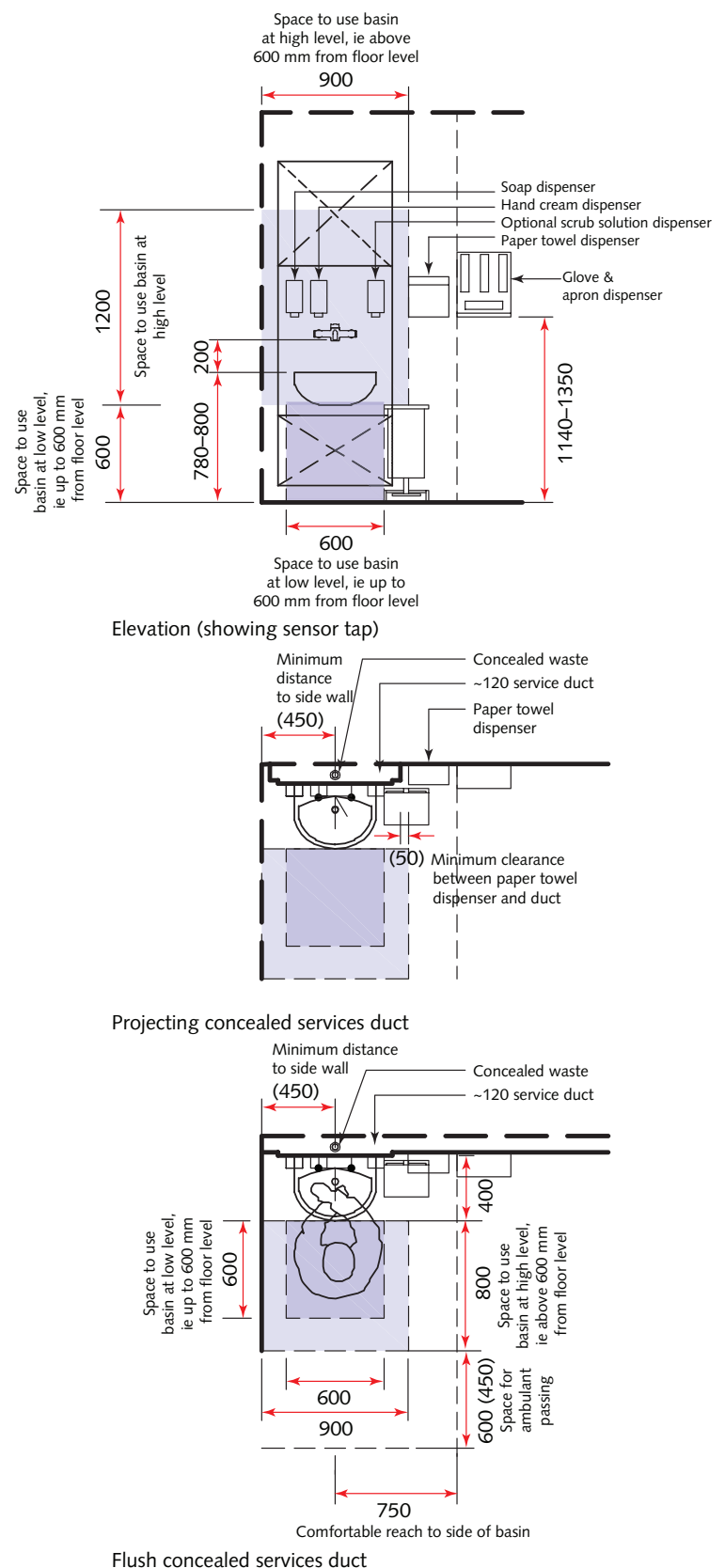
Figure 70 Space requirements for standing use of a clinical wash-hand basin assembly
