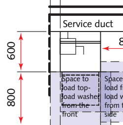
Top-loading washer/macerator
