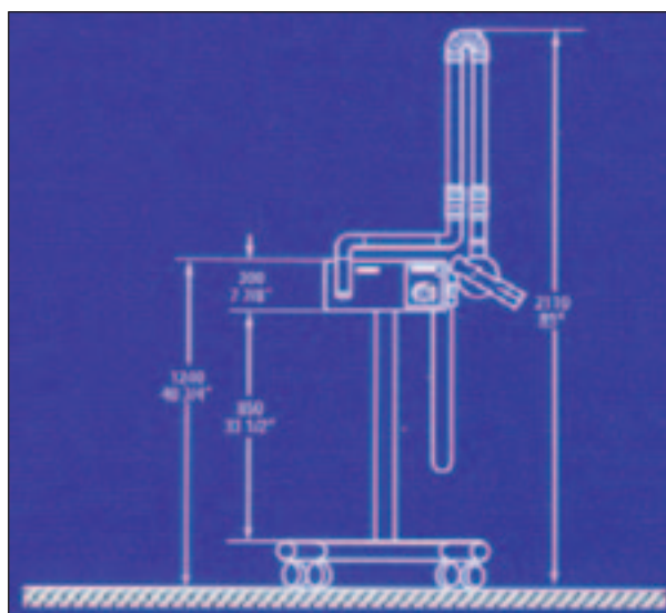
Figure 1.3 Example of mobile extra-oral unit, courtesy Sirona Dental Systems, a division of Siemens Medical Solutions
