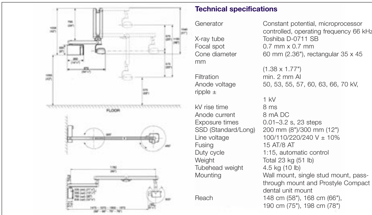
Figure 1.2 Example dimensions for a typical extra-oral X-ray unit, courtesy Planmeca
