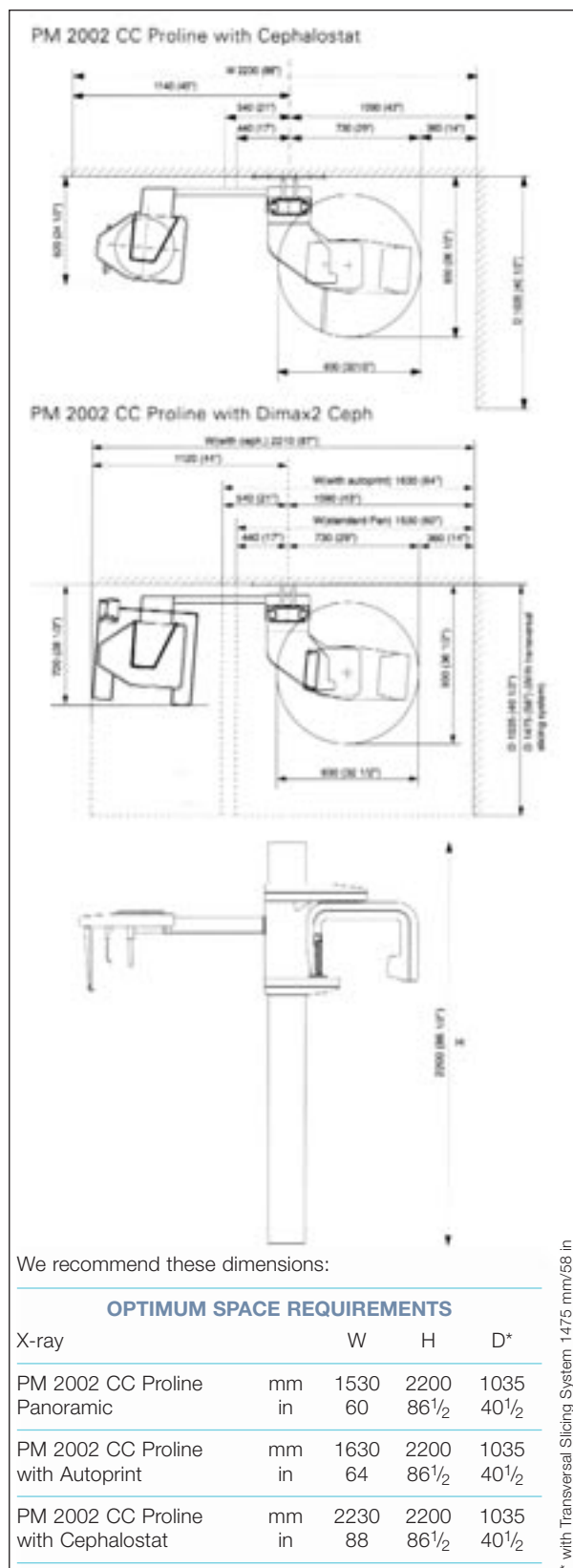
Figure 1.5 Example dimensions of an OPG/dental panoramic unit fitted with cephalostat attachment, courtesy Planmeca
