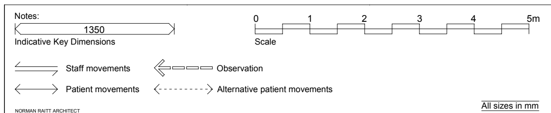
PLAN 29 MULTI-CUBICLE ULTRASOUND SUITE Access and movement / key to clinical equipment
