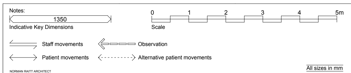
PLAN 25 P.E.T. SCANNER SUITE Access and movement / Clinical equipment
