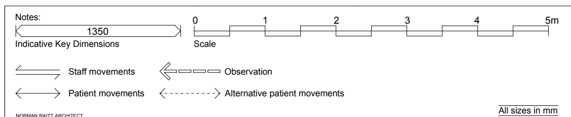
PLAN 23 GAMMA CAMERA ROOM WITH INJECTION AREA ELSEWHERE IN SUITE Movement and observation
