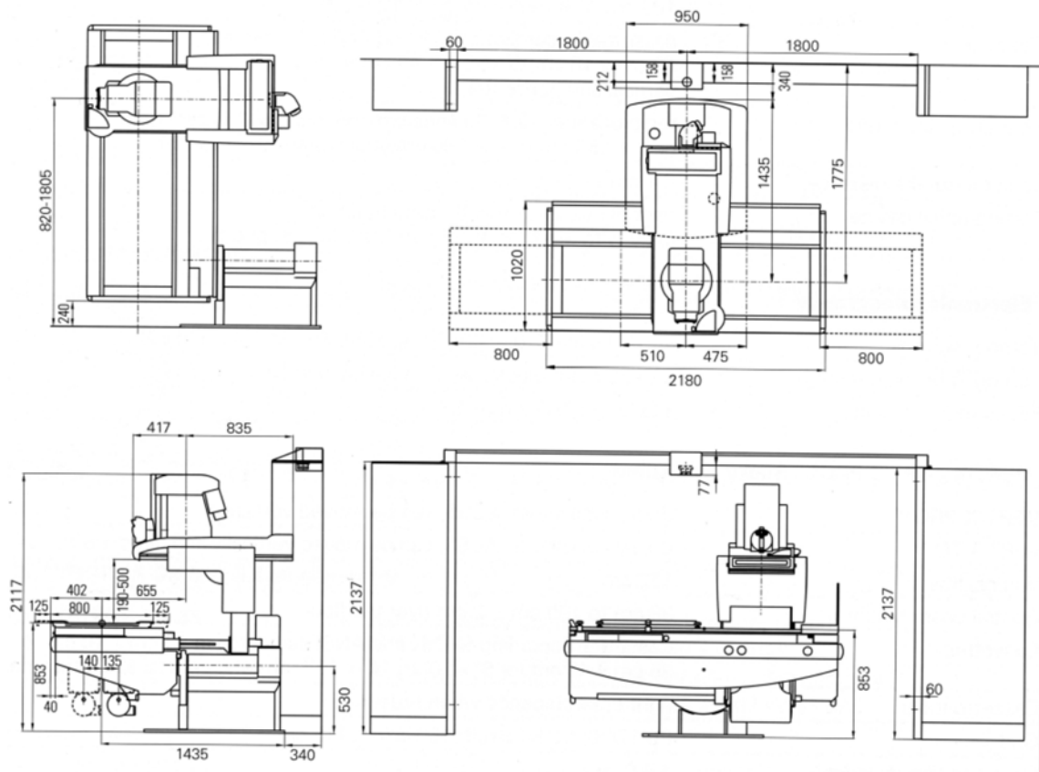
Figure 5.1: Example dimensions for a conventional/universal fluoroscopy unit
