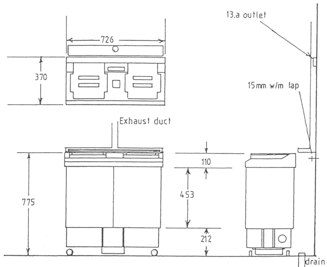
Figure 3.2: An example of chemical mixing device
