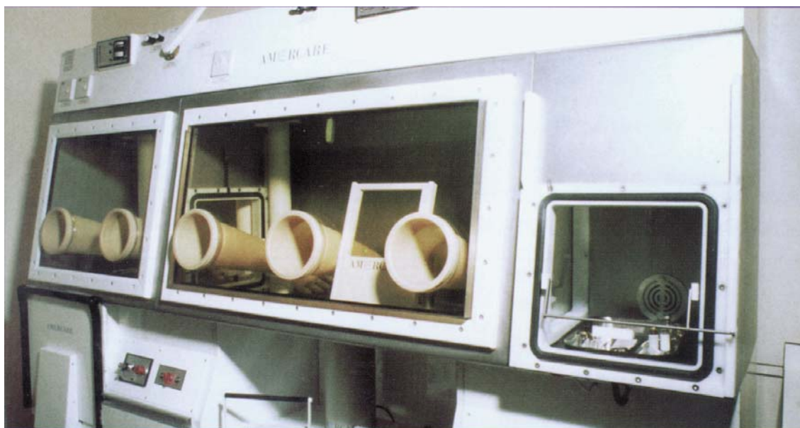
Figure 8.3: Class (iii) microbiological safety cabinet used in the preparation of radiopharmaceuticals
