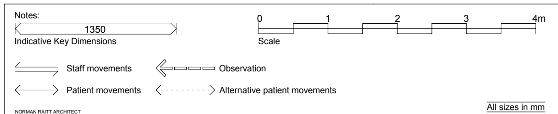
PLAN 5 COMPUTED RADIOGRAPHY (C.R.) Key to equipment in PLAN 4
