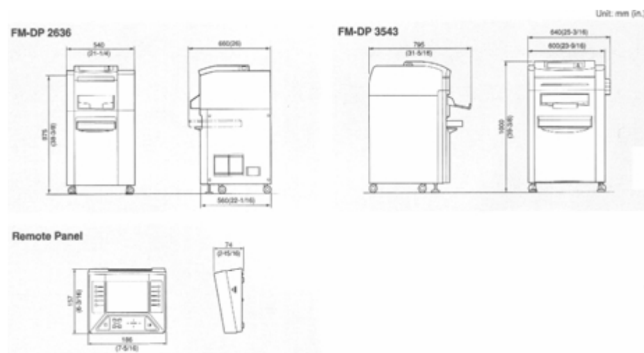
Figure 3.4: Example of a free-standing dry laser image Image reproduced by courtesy of Fuji Medical Systems
