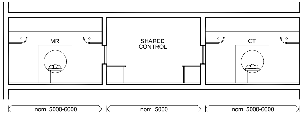
SECTION - A
