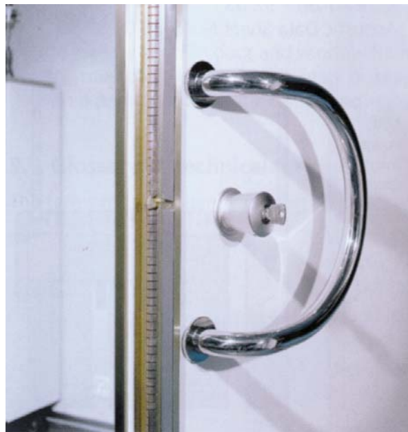
Figure 13.4: Engineering for the integration of a radio frequency shielded door
