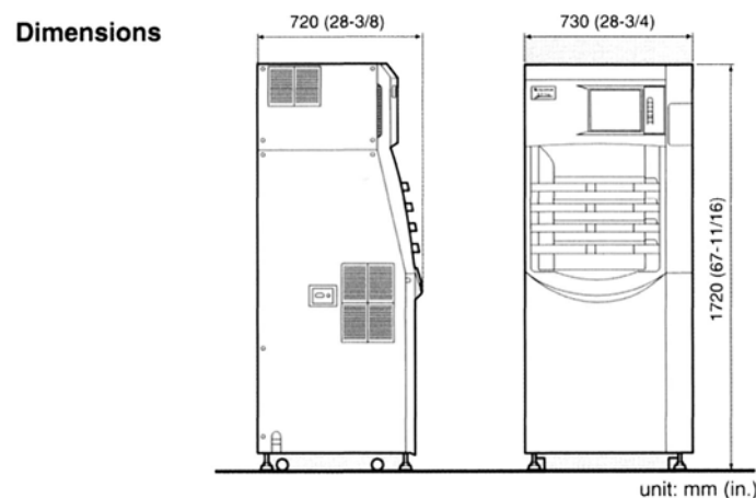
Figure 3.6: Large high-throughput Computed Radiography Unit
