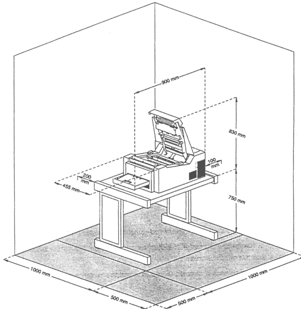
Figure 3.3 Example of a desktop dry laser printing device
