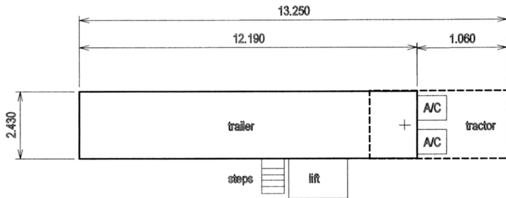
PLAN SHOWING OVERALL DIMENSIONS AND PATIENT ENTRANCE
