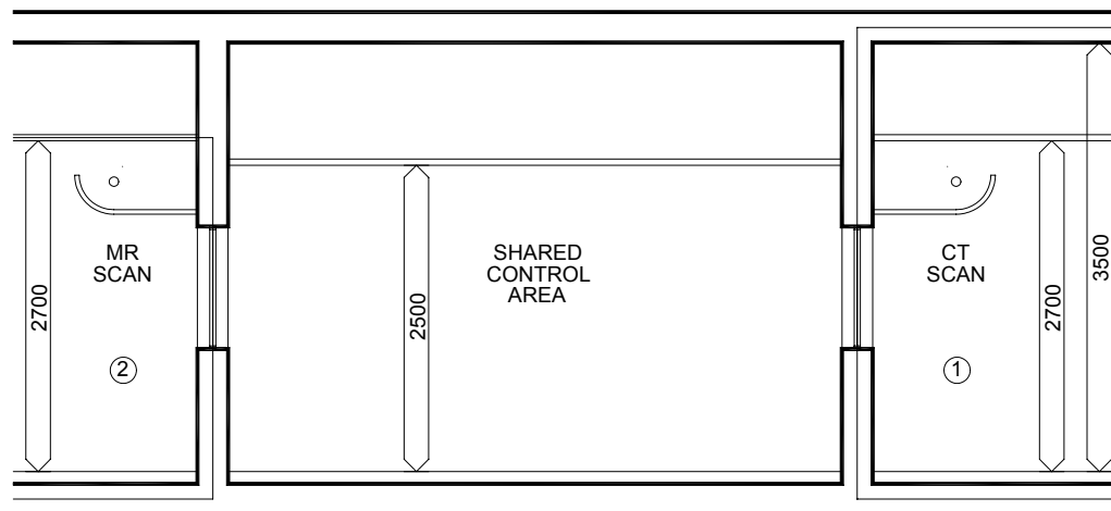
SECTION - B
