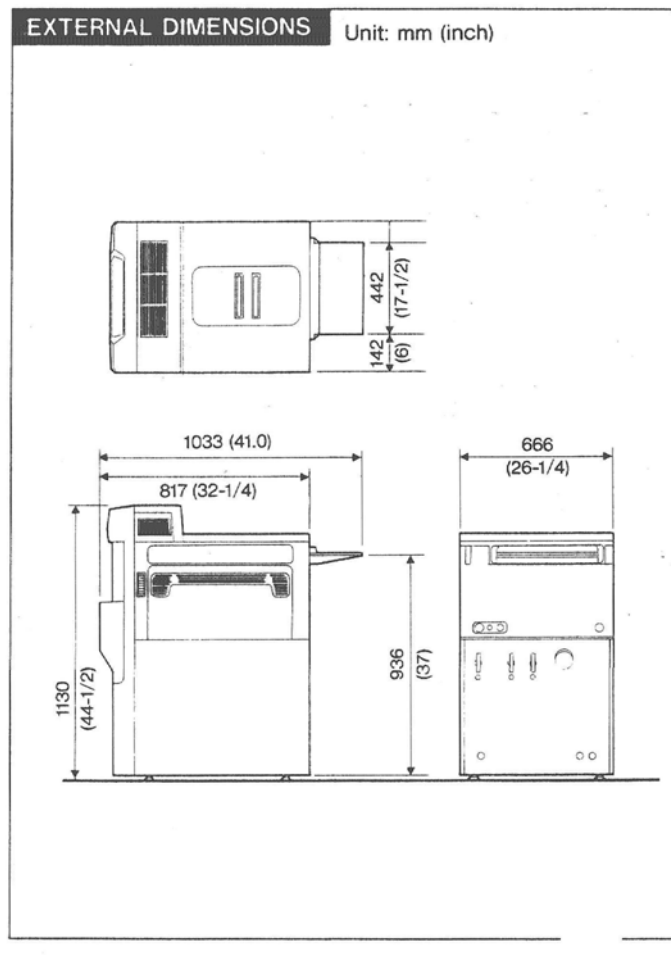
Figure 3.1: Example of a conventional film processing unit for use in a darkroom
