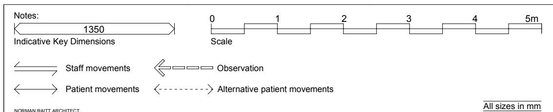
PLAN 30 SINGLE ULTRASOUND ROOM PLANNED / EQUIPPED FOR ROUTINE EXAMINATIONS AND MINOR INTERVENTIONAL PROCEDURES Access and movement / key to clinical equipment
