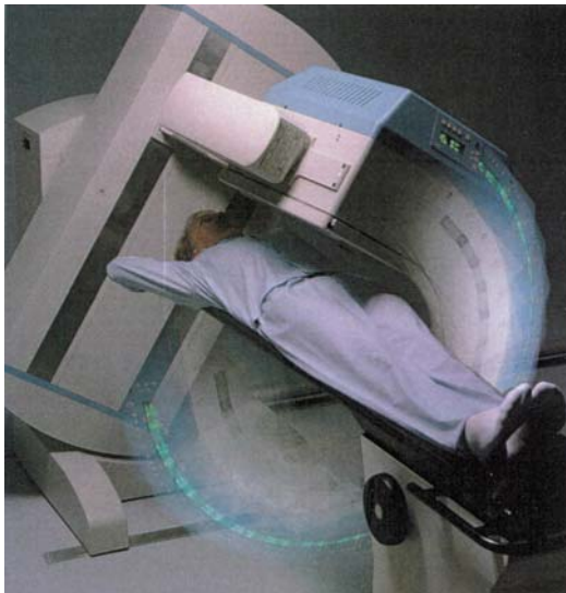
Figure 8.1: Example of a single detector gamma camera and its movement during SPECT acquisitions
