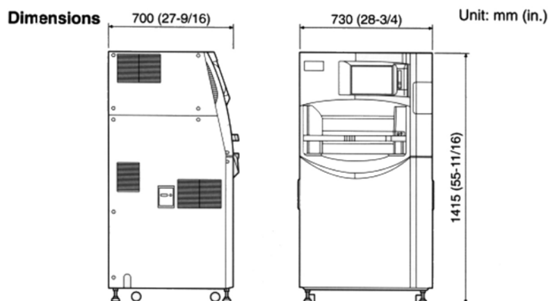
Figure 3.7: Low/medium-throughput Computed Radiography Unit
