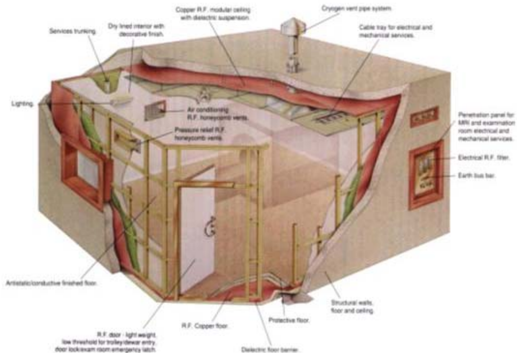
Figure 13.3: Image of a typical MRI scanner room
