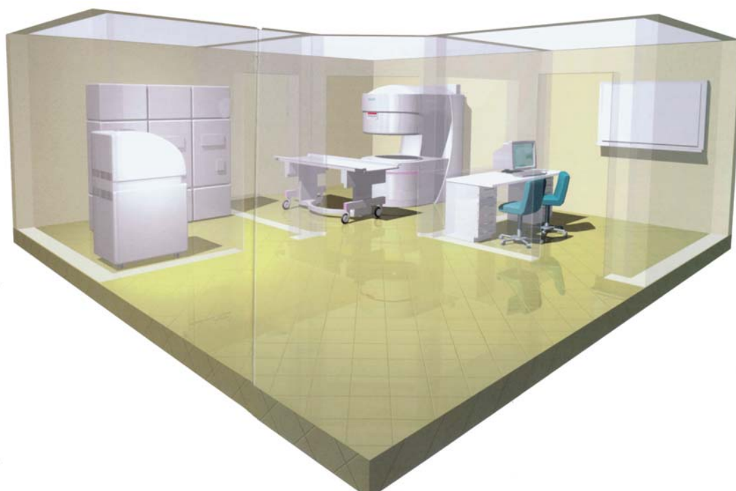
Figure 13.2: Idealised layout of an open MRI system allowing for imaging procedures only
