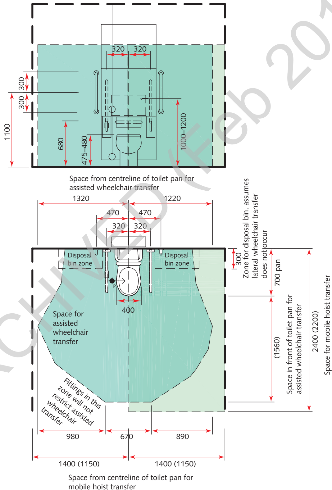
Figure 90 Space requirements for assisted toilet
