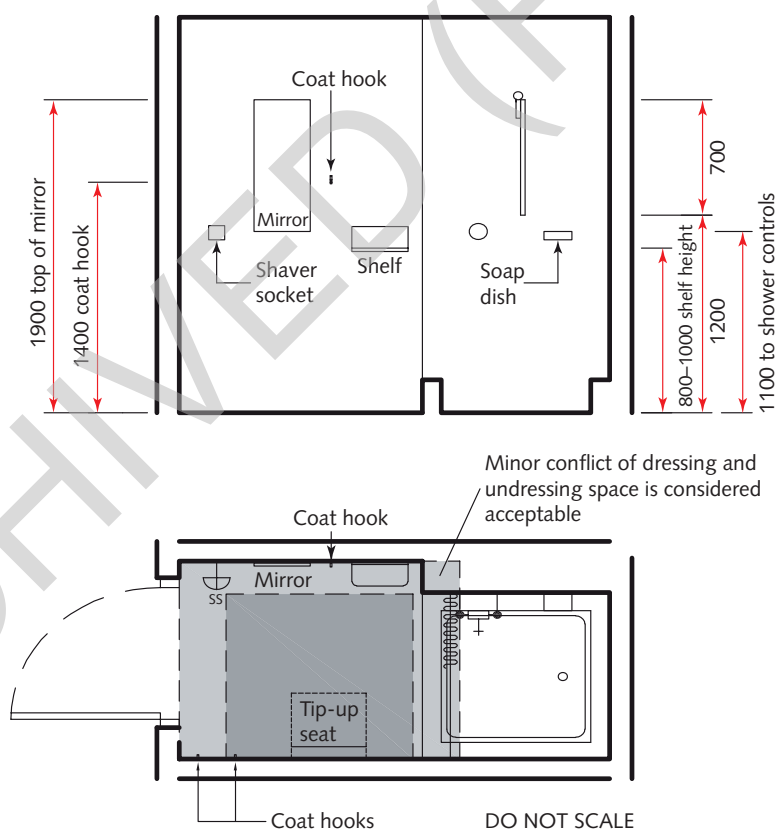
Figure 46 Space requirements for ambulant shower room
