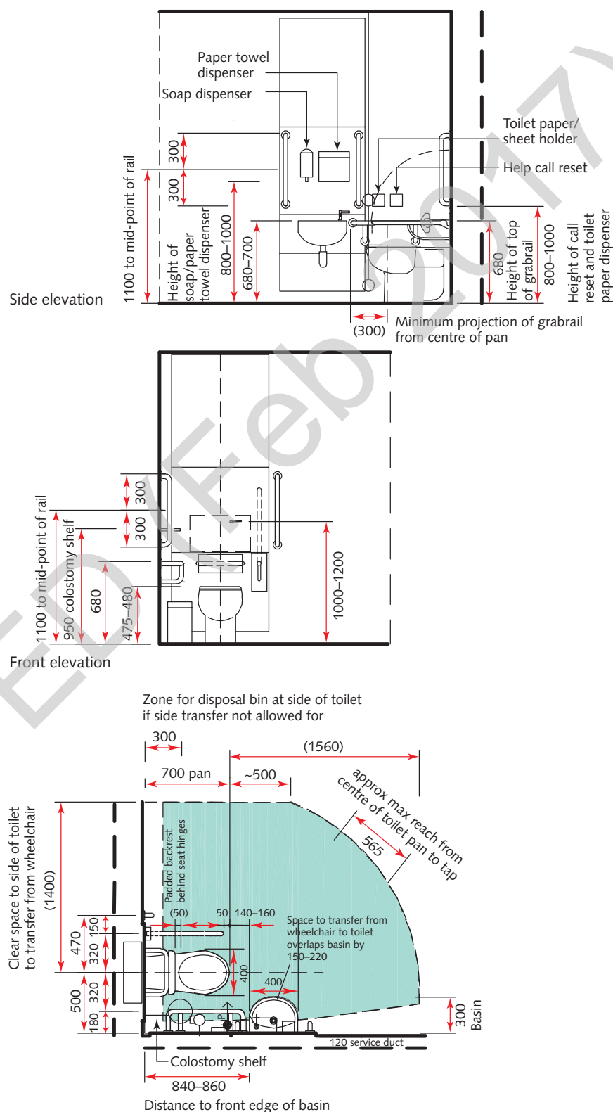
Figure 68 Space requirements for an independent wheelchair toilet and adjacent hand-rinse basin
