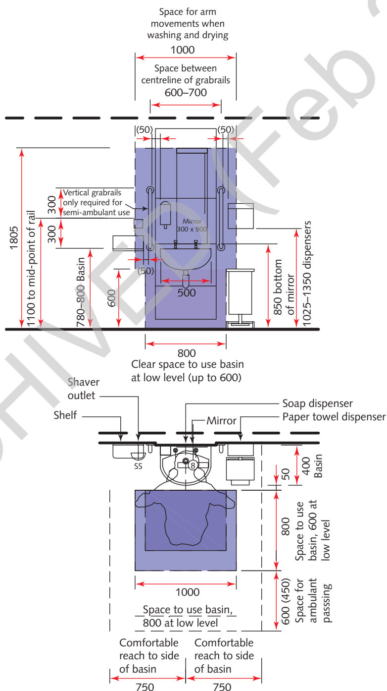
Figure 5 Space requirements for ambulant/semi-ambulant use of a 400 mm deep × 500 mm wide wash-hand basin
