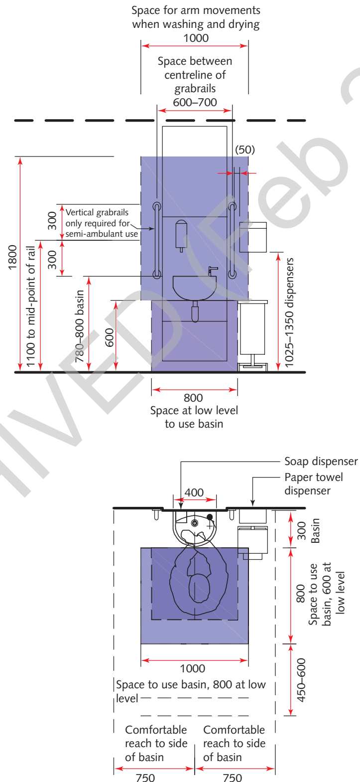
Figure 88 Space requirements for 300 mm deep hand-rinse basin suitable for ambulant and semi-ambulant use
