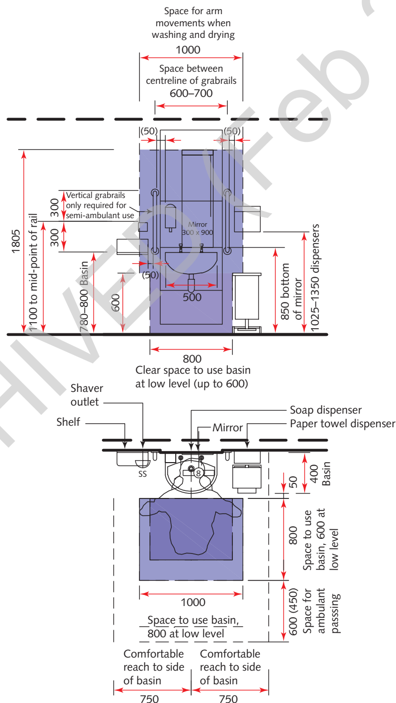
Figure 96 Space requirements for ambulant/semi-ambulant use of 400 mm deep \times 500 mm wide wash-hand basin
