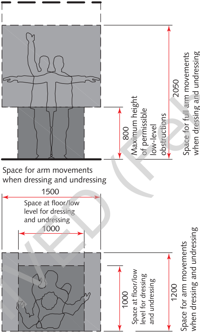
Figure 3 Space requirements for ambulant dressing and undressing
