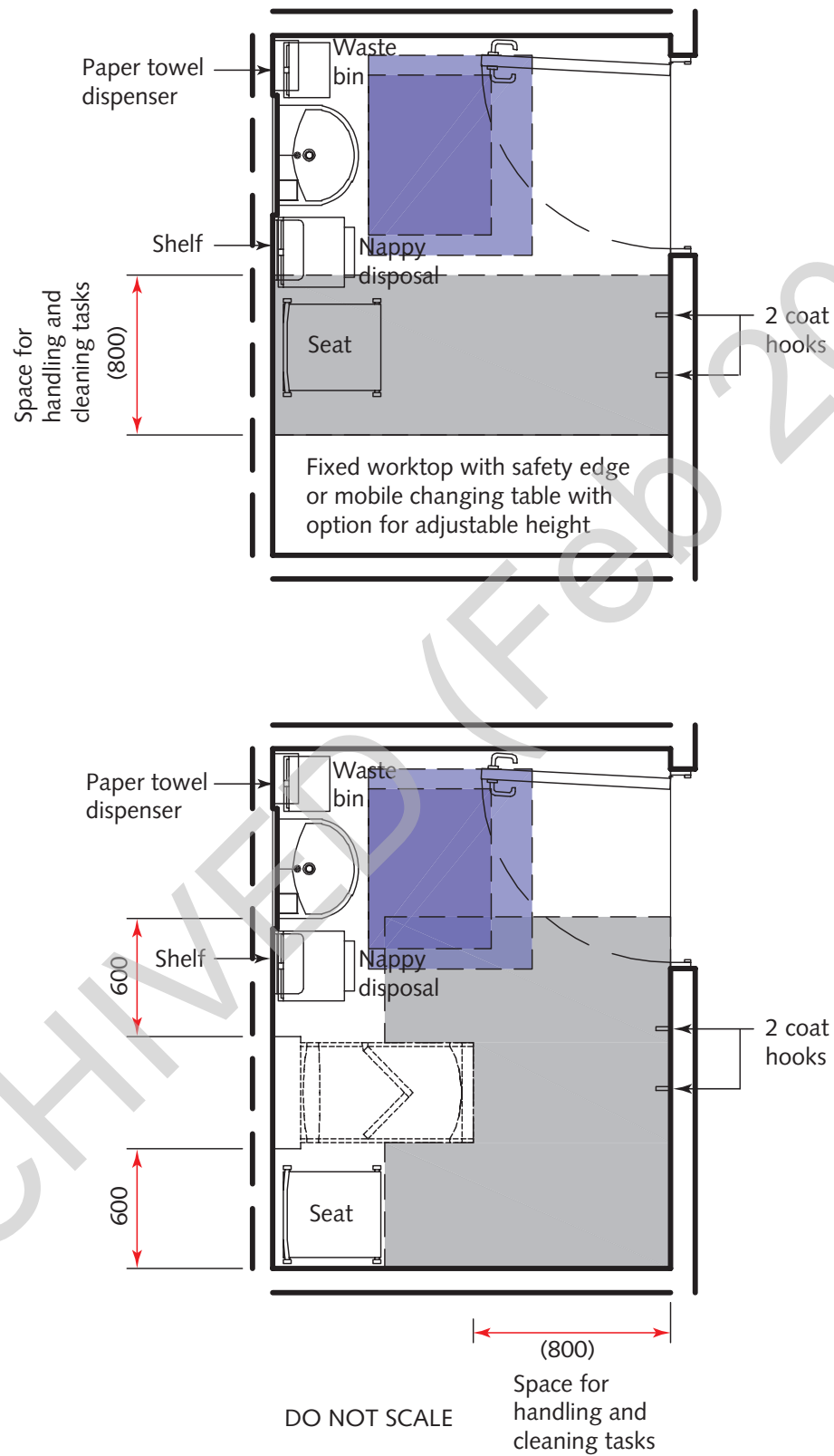
Figure 43 Space requirements for nappy changing room
