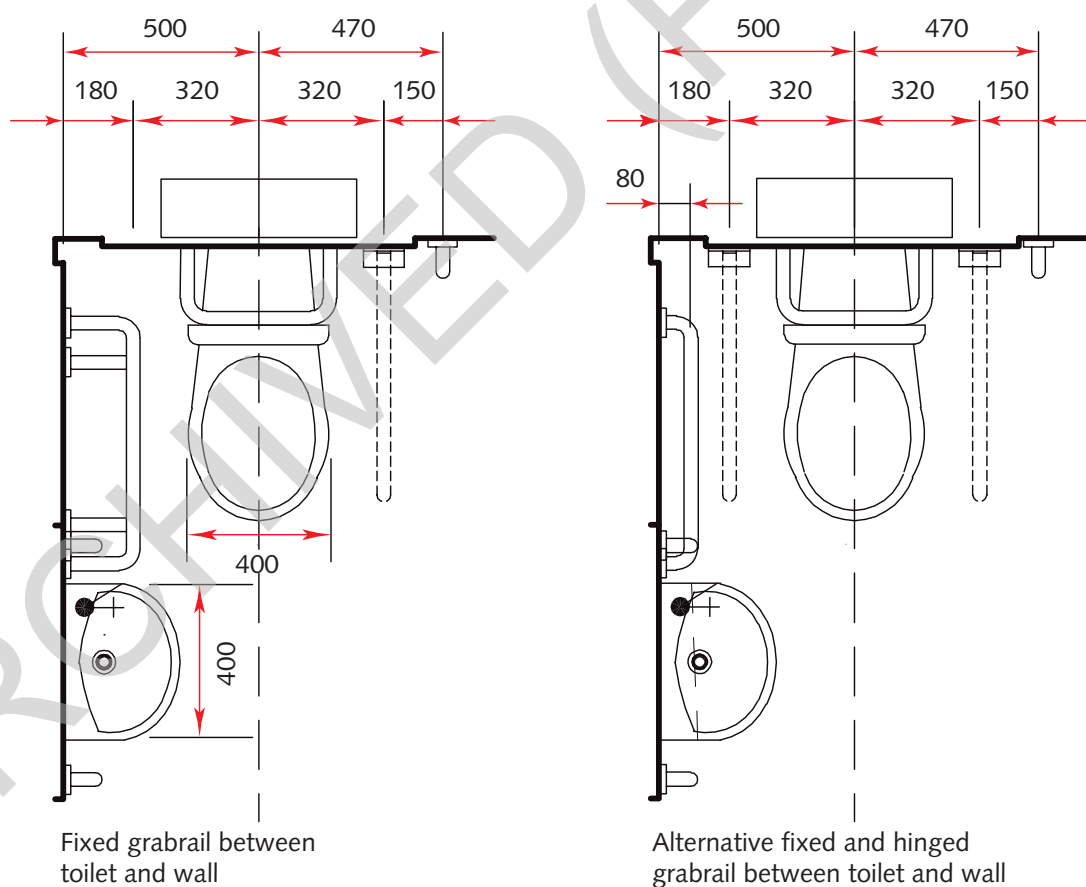
Figure 95 Space requirements showing fixing position of grabrails for independent wheelchair toilet and adjacent hand-rinse basin
