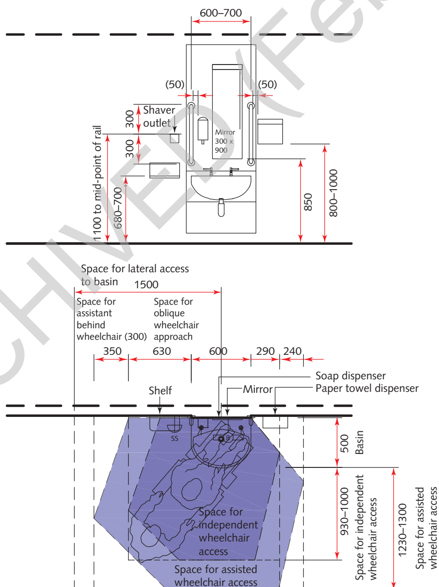
Figure 51 Space requirements for wheelchair accessible wash-hand basin, suitable for seated use
