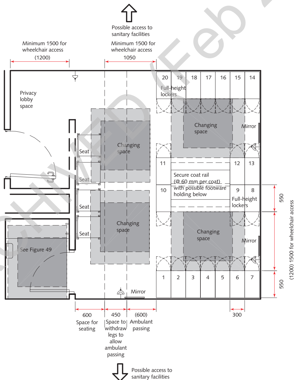
Figure 25 Space requirements for changing area: staff, 20 lockers
