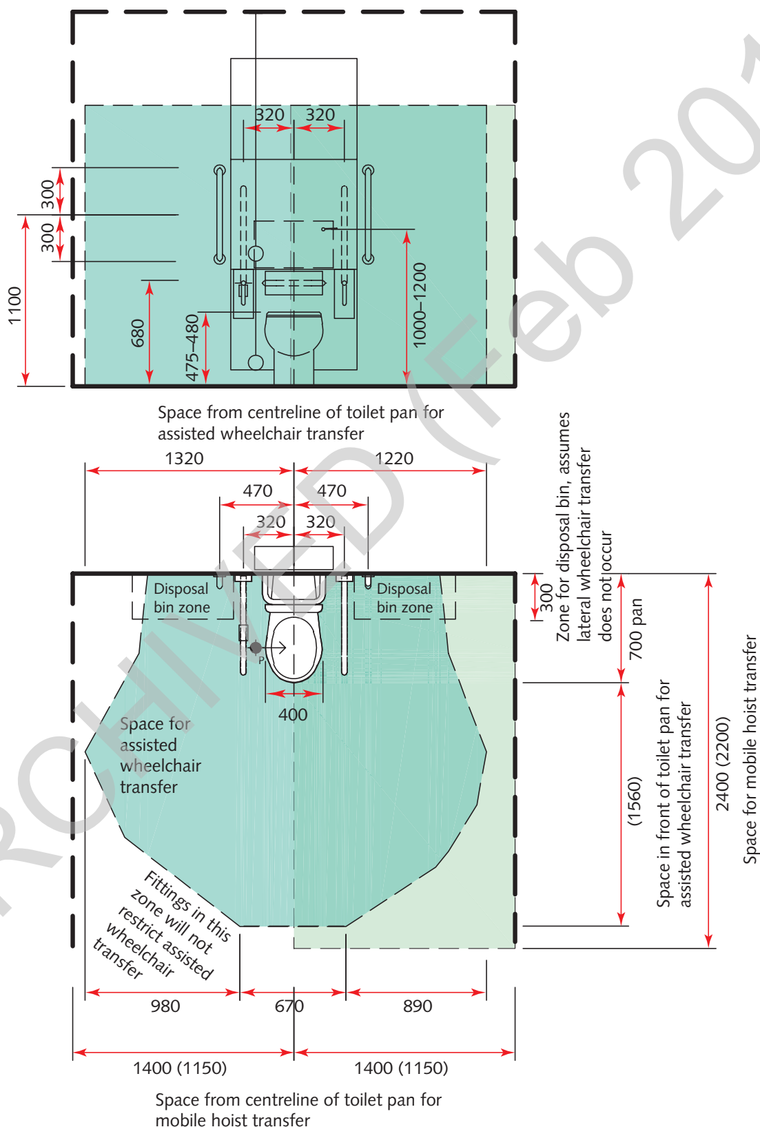
Figure 10 Space requirements to access an assisted toilet
