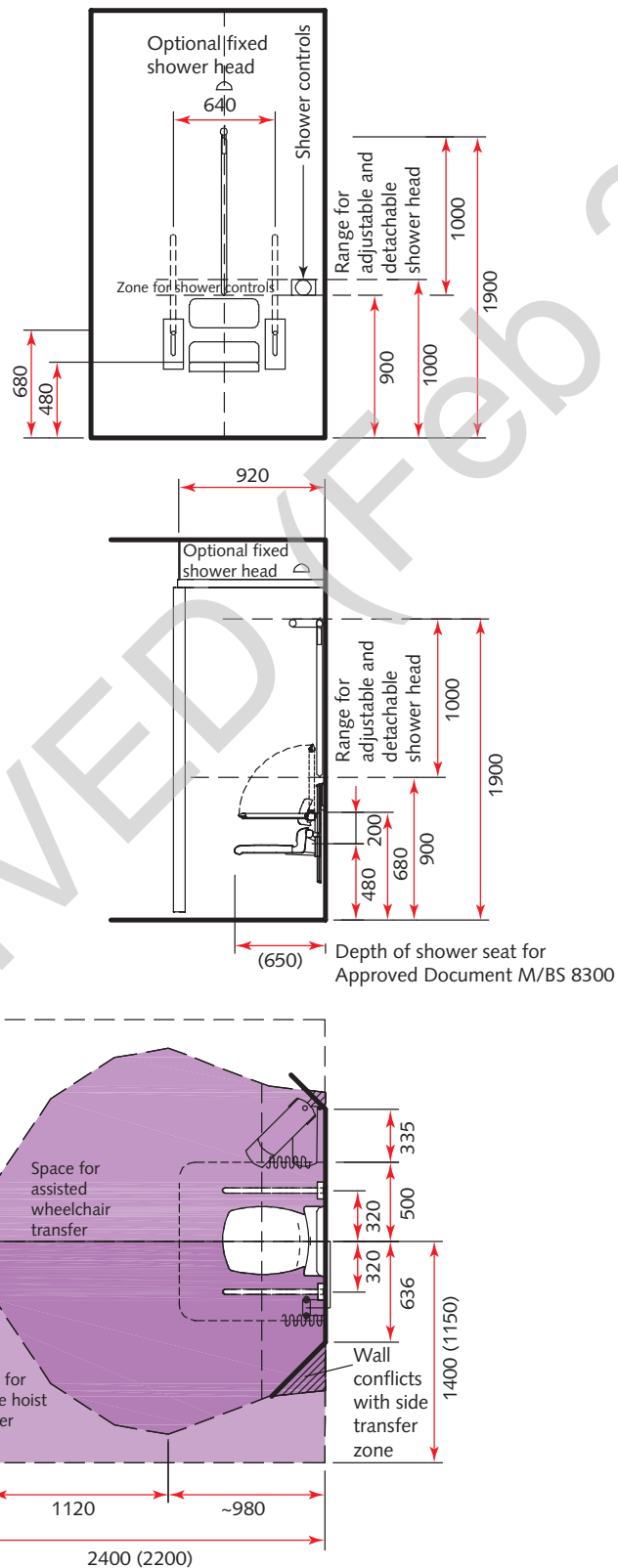
Figure 58 Space requirements for shower for use in chamfered en-suite shower room
