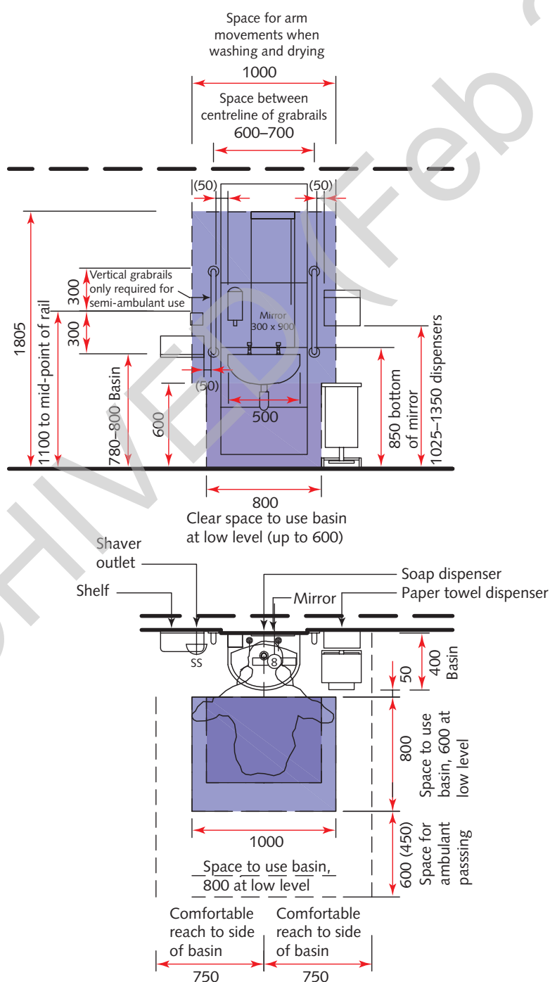
Figure 37 Space requirements for ambulant/semi-ambulant use of a 400 mm deep × 500 mm wide wash-hand basin
