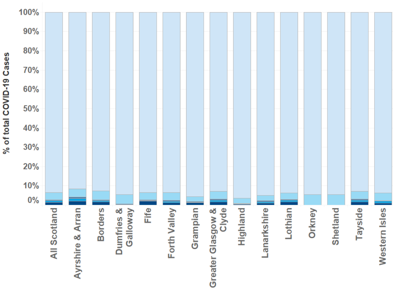
Figure 2: Proportion of COVID-19 cases by onset status and NHS board: specimen dates up to 6 June 2021. 1,2,3
