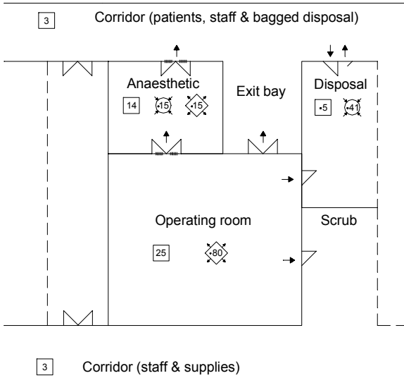
Plan 3 Linked corridor with external scrub and remote sterile pack store
