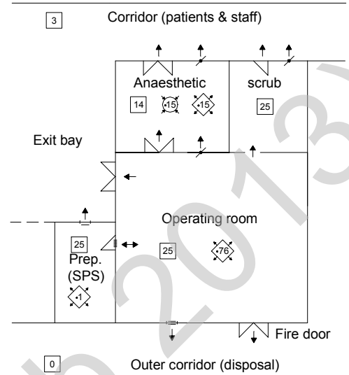
Plan 4 Two corridor sterile pack store with disposal hatch
