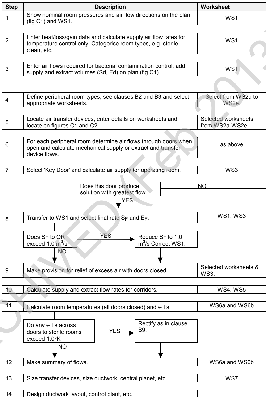
Figure A1: Air flow design procedures
