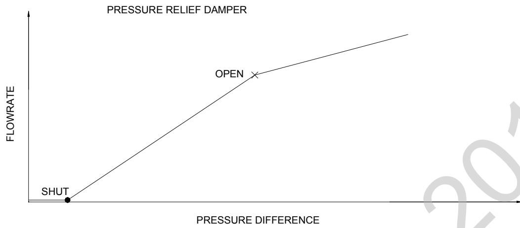
Figure B1: Typical flow rate / pressure characteristics
