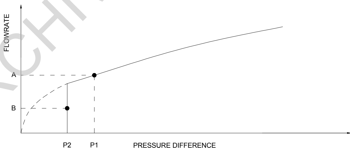
Figure B2: Pressure stabilisers performing two tasks
